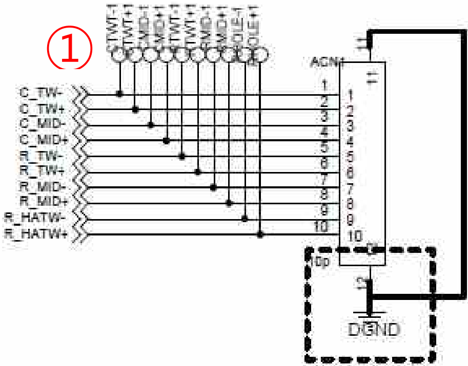
CT+RIGHT 5 SPK.
